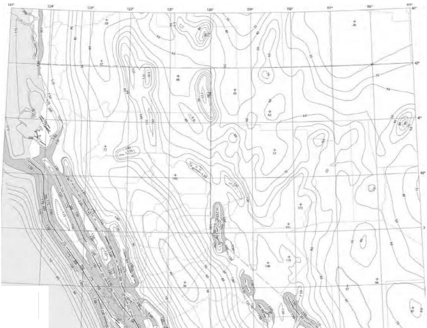
FIGURE 10-10.5(b) MAXIMUM CONSIDERED EARTHQUAKE GROUND MOTION FOR REGION 1 OF 0.2 SEC SPECTRAL RESPONSE ACCELERATION (5% OF CRITICAL DAMPING), SITE CLASS B
