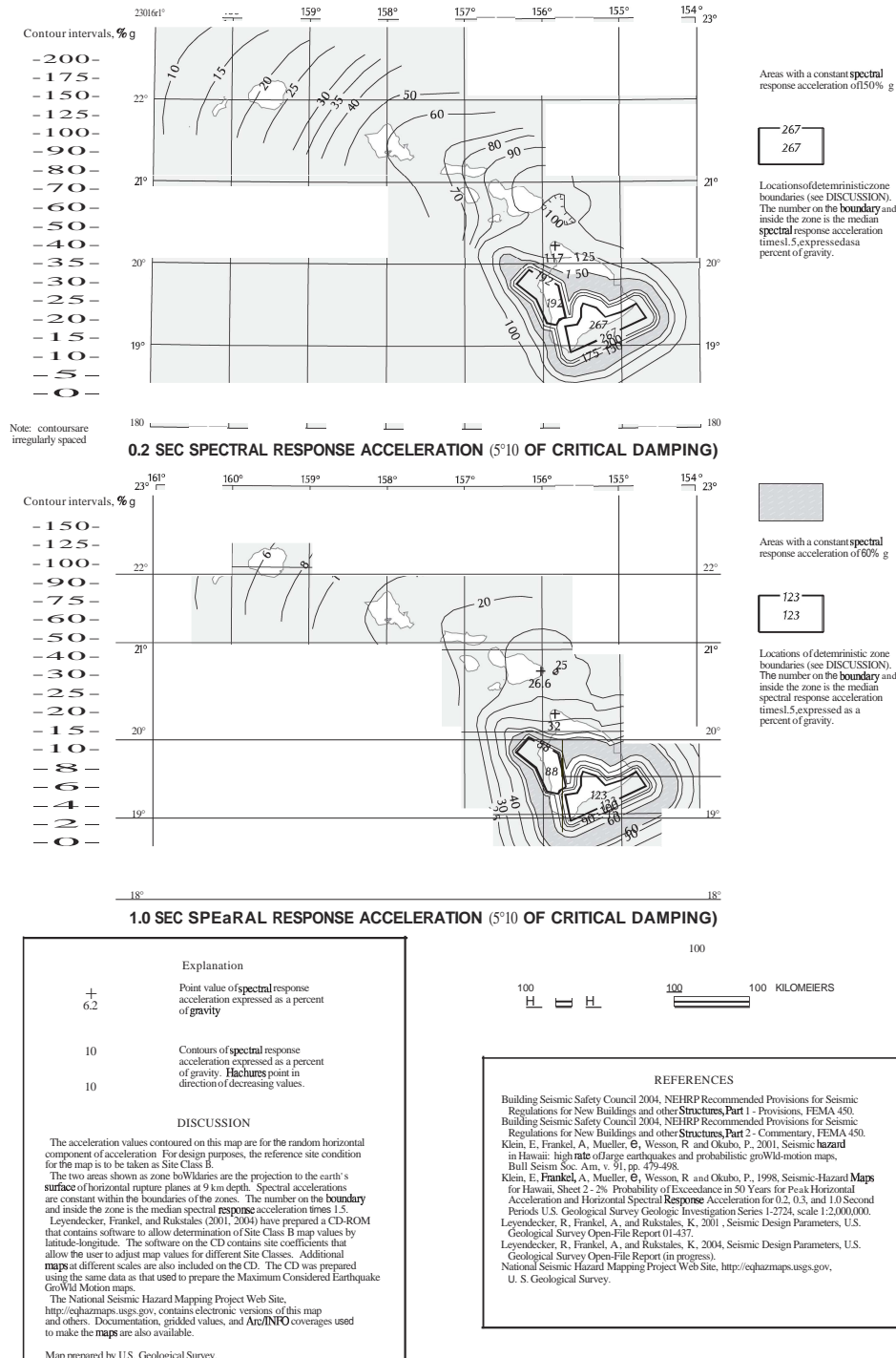
FIGURE 1613.5(10) MAXIMUM CONSIDERED EARTHQUAKE GROUND MOTION FOR HAWAII FOR 0.2 AND 1.0 SEC SPECTRAL RESPONSE ACCELERATION (5% OF CRITICAL DAMPING), SITE CLASS B
