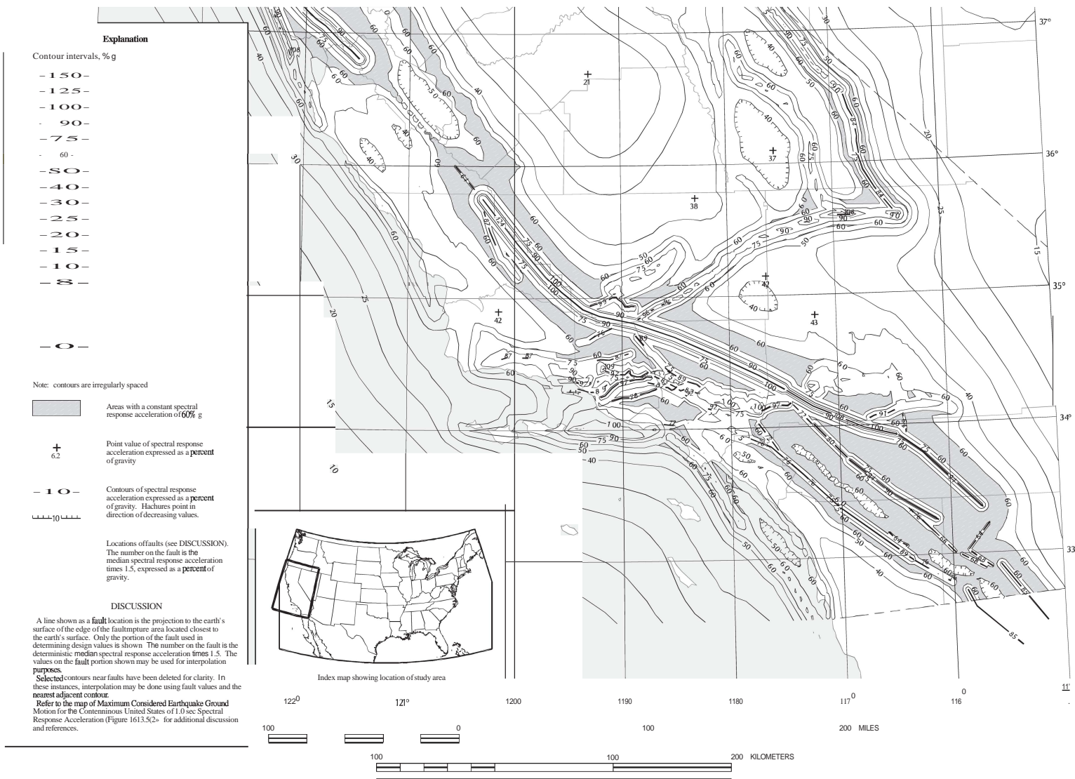
FIGURE 1613.5(4)-continued MAXIMUM CONSIDERED EARTHQUAKE GROUND MOTION FOR REGION 1 OF 1.0 SEC SPECTRAL RESPONSE ACCELERATION (5% OF CRITICAL DAMPING), SITE CLASS B
