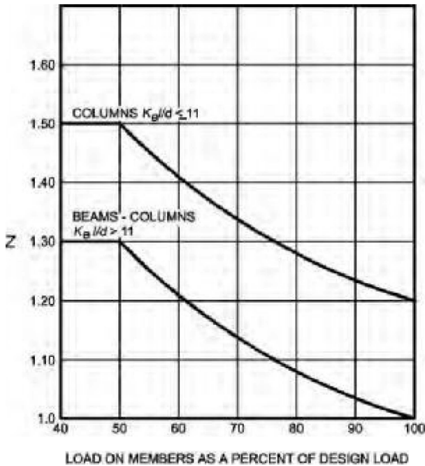
FIGURE 721.6.3(1) LOAD FACTOR
