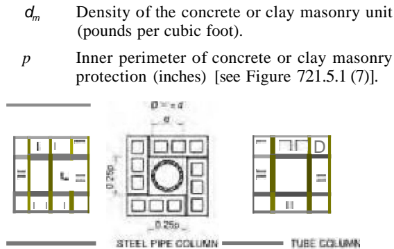
FIGURE 721.5.1(7) CONCRETE OR CLAY MASONRY PROTECTED STRUCTURAL STEEL COLUMNS
