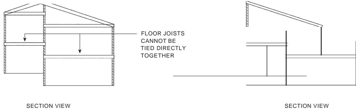
FIGURE 2308.12.6(6) PORTIONS OF FLOOR LEVEL OFFSET VERTICALLY
